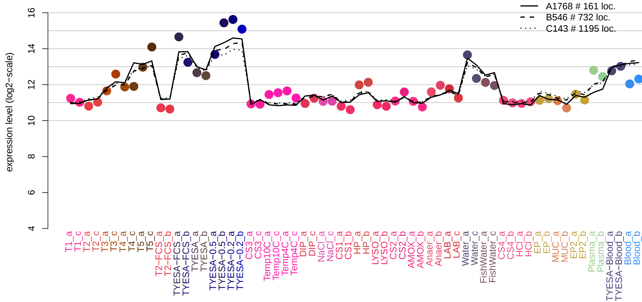
THC0290_0243 rbfA (298577,298969,1)
