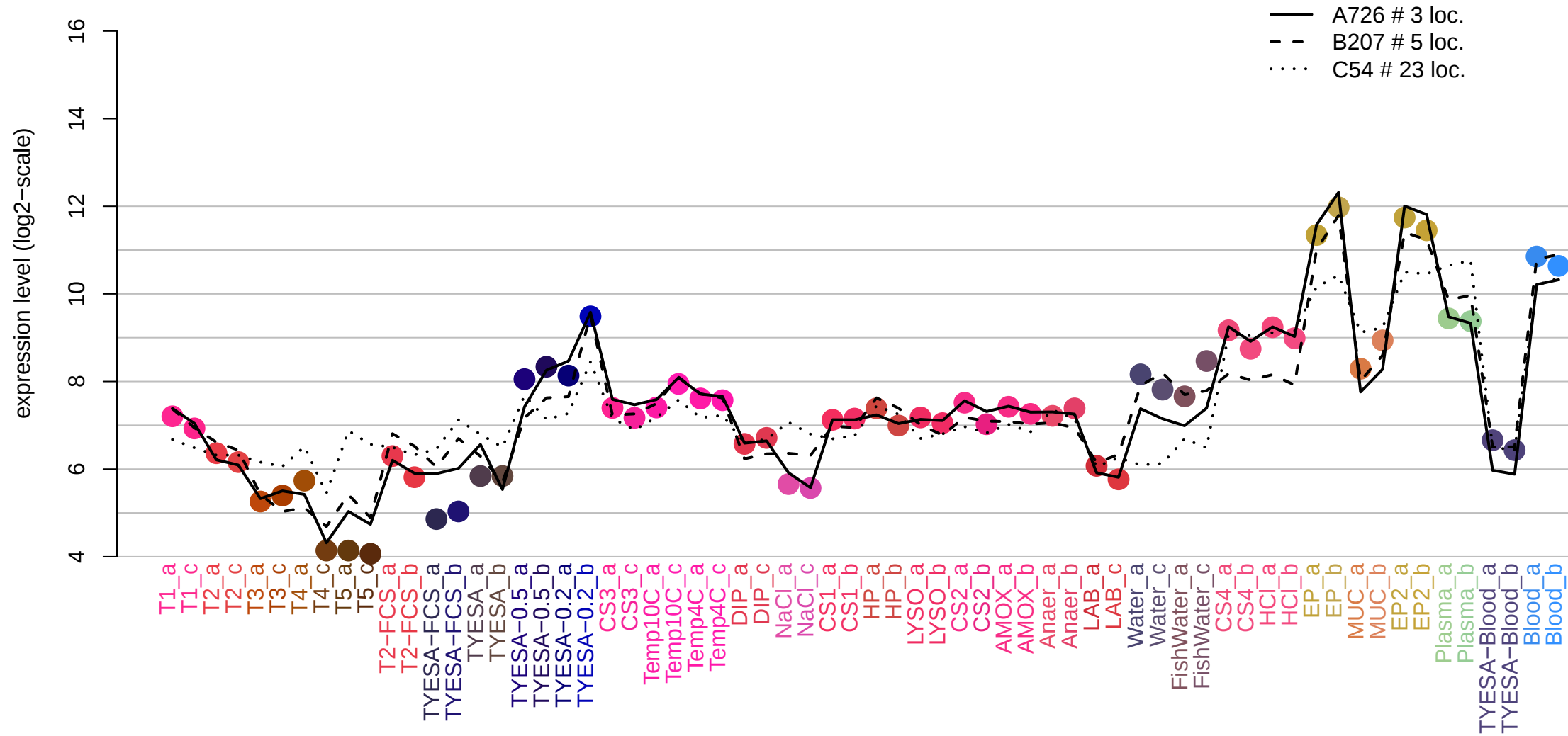
THC0290_0263 metY (319731,321023,-1)
