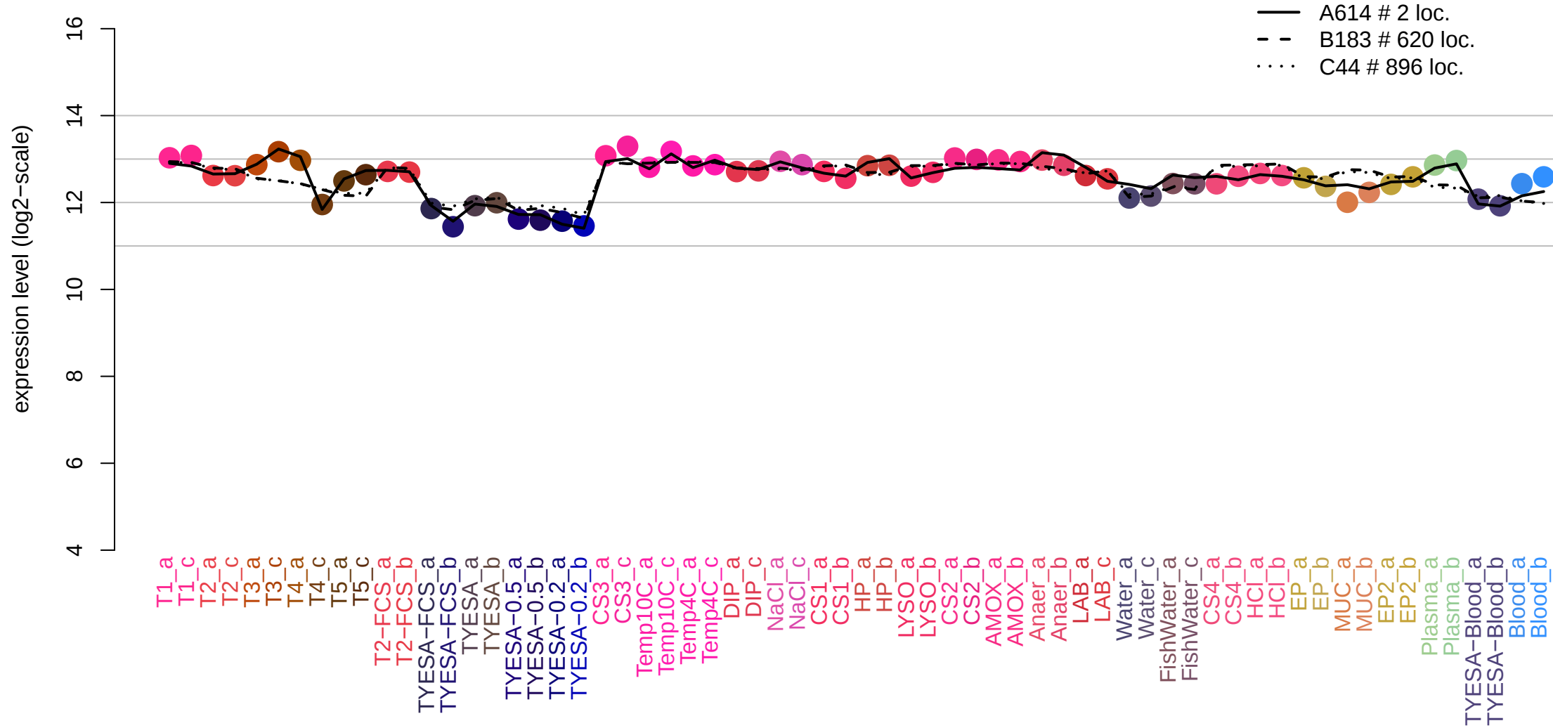
THC0290_0661 ftsA (797014,798414,1)
