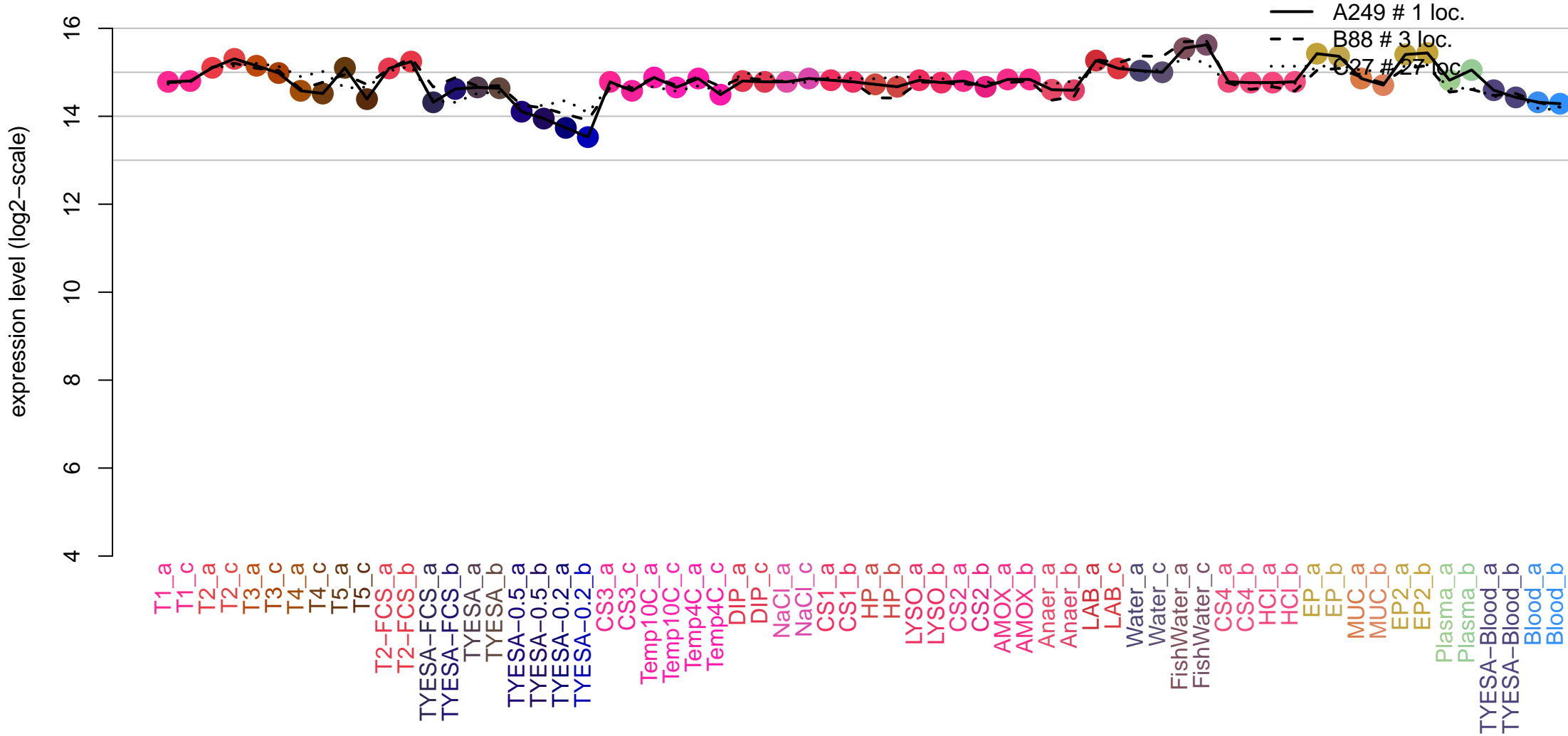
THC0290_0742 gldM (881104,882633,1)
