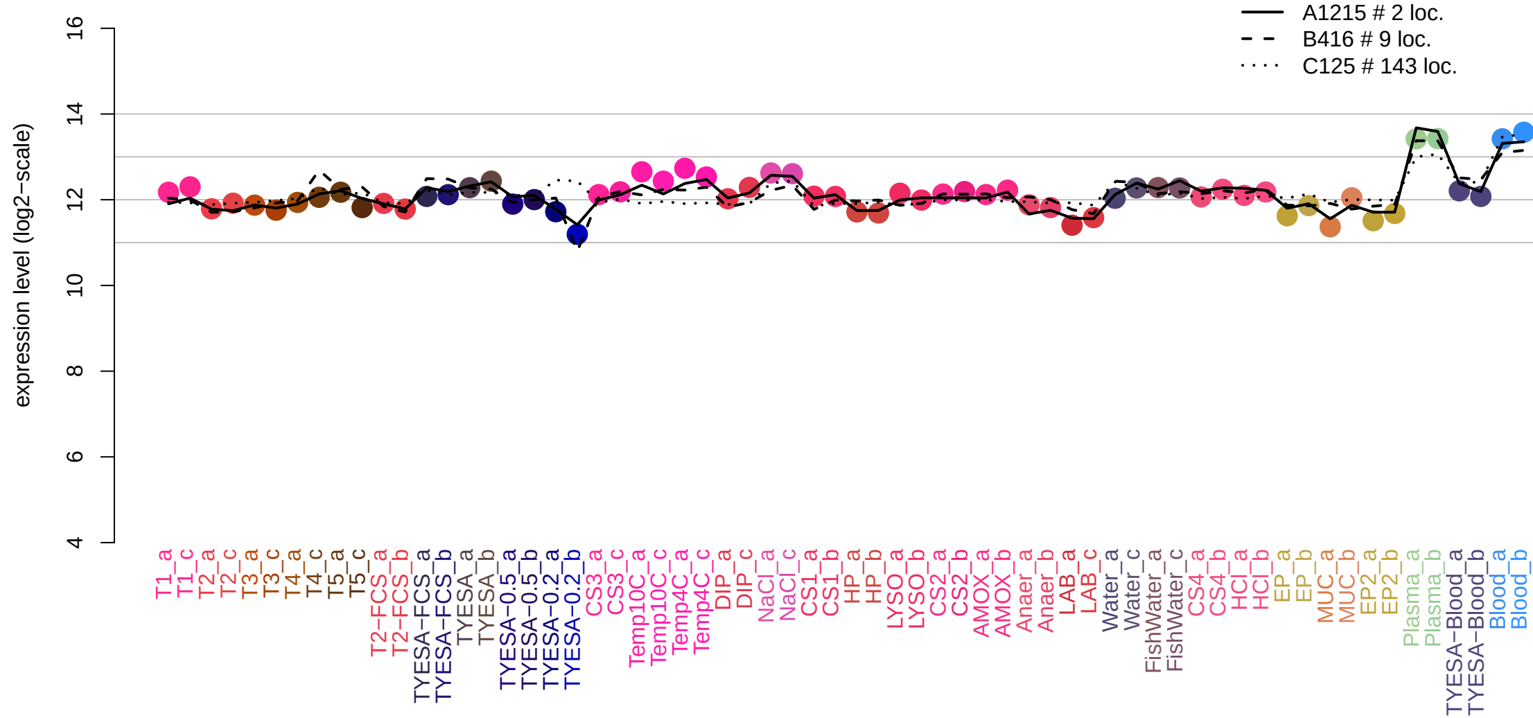
THC0290_0813 purA (968364,969635,1)
