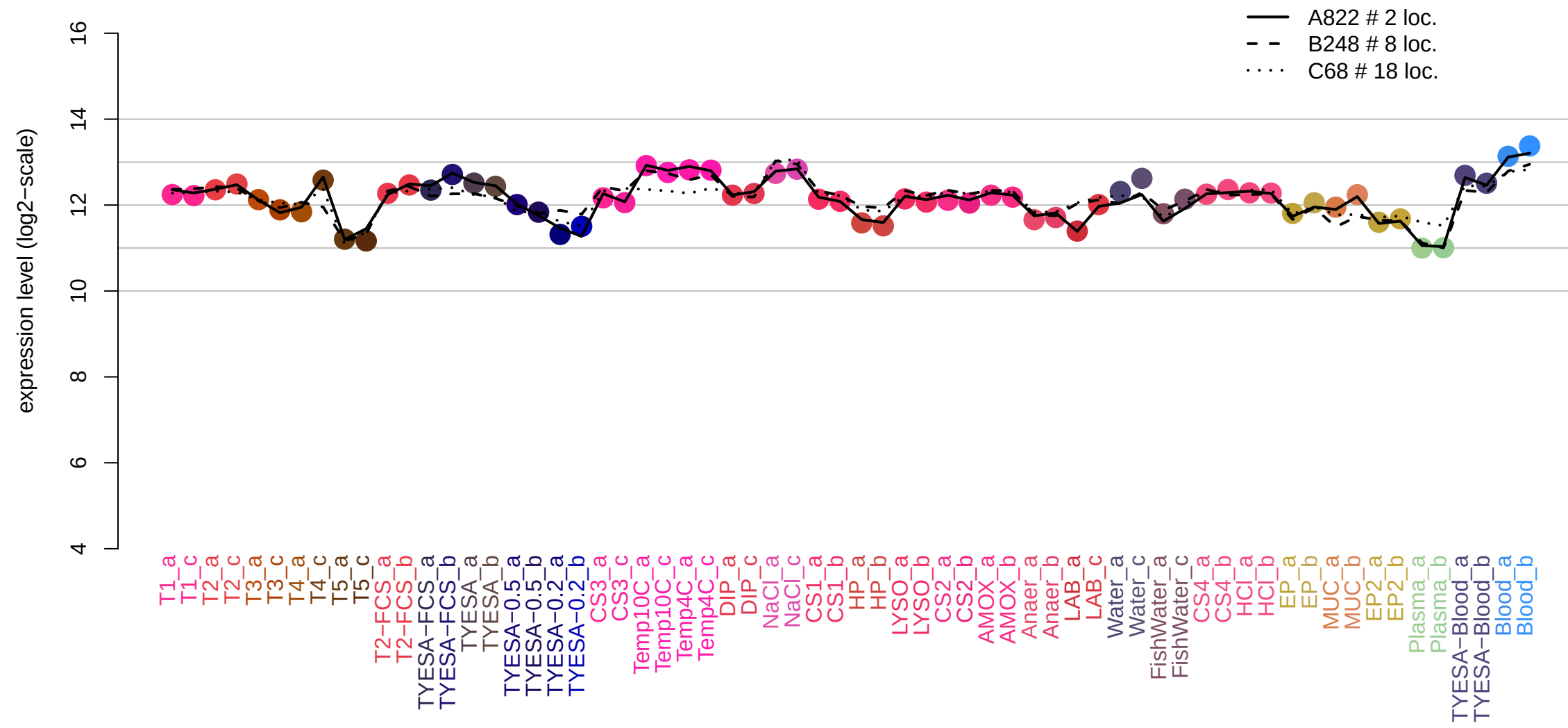
THC0290_0872 dapA (1029395,1030276,-1)
