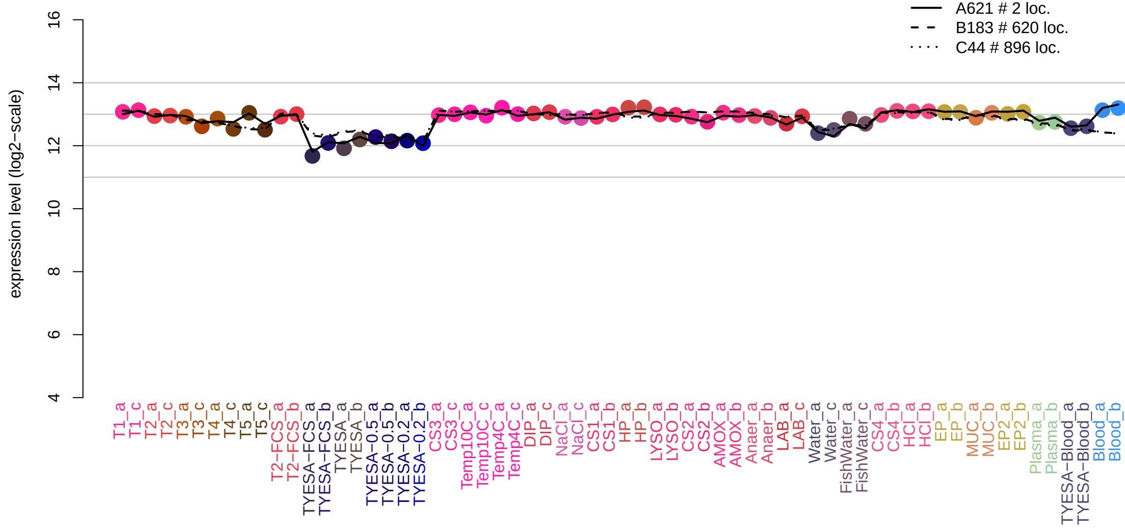
THC0290_1012 aspC2 (1192373,1193563,1)
