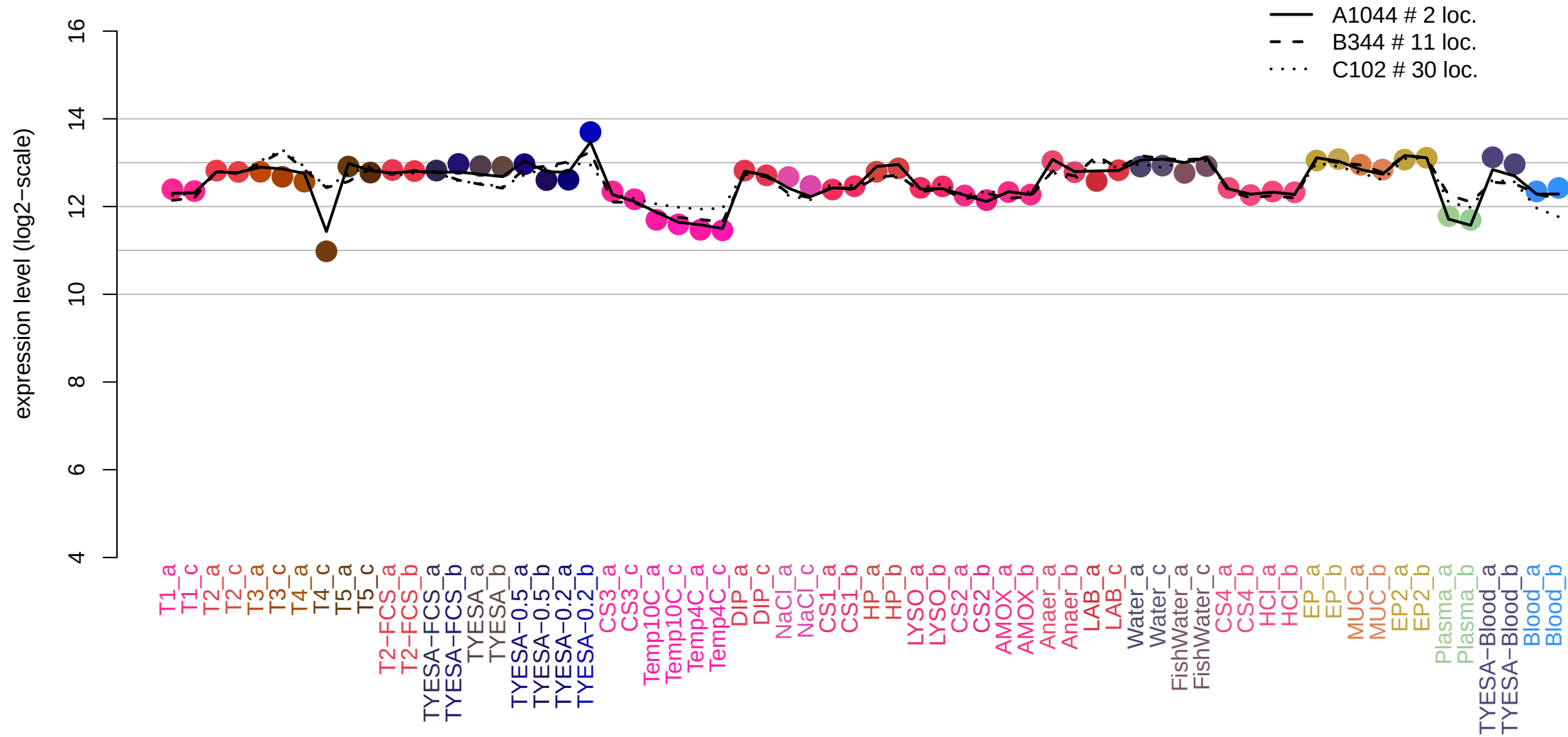
THC0290_1095 pfkA (1278886,1279872,1)
