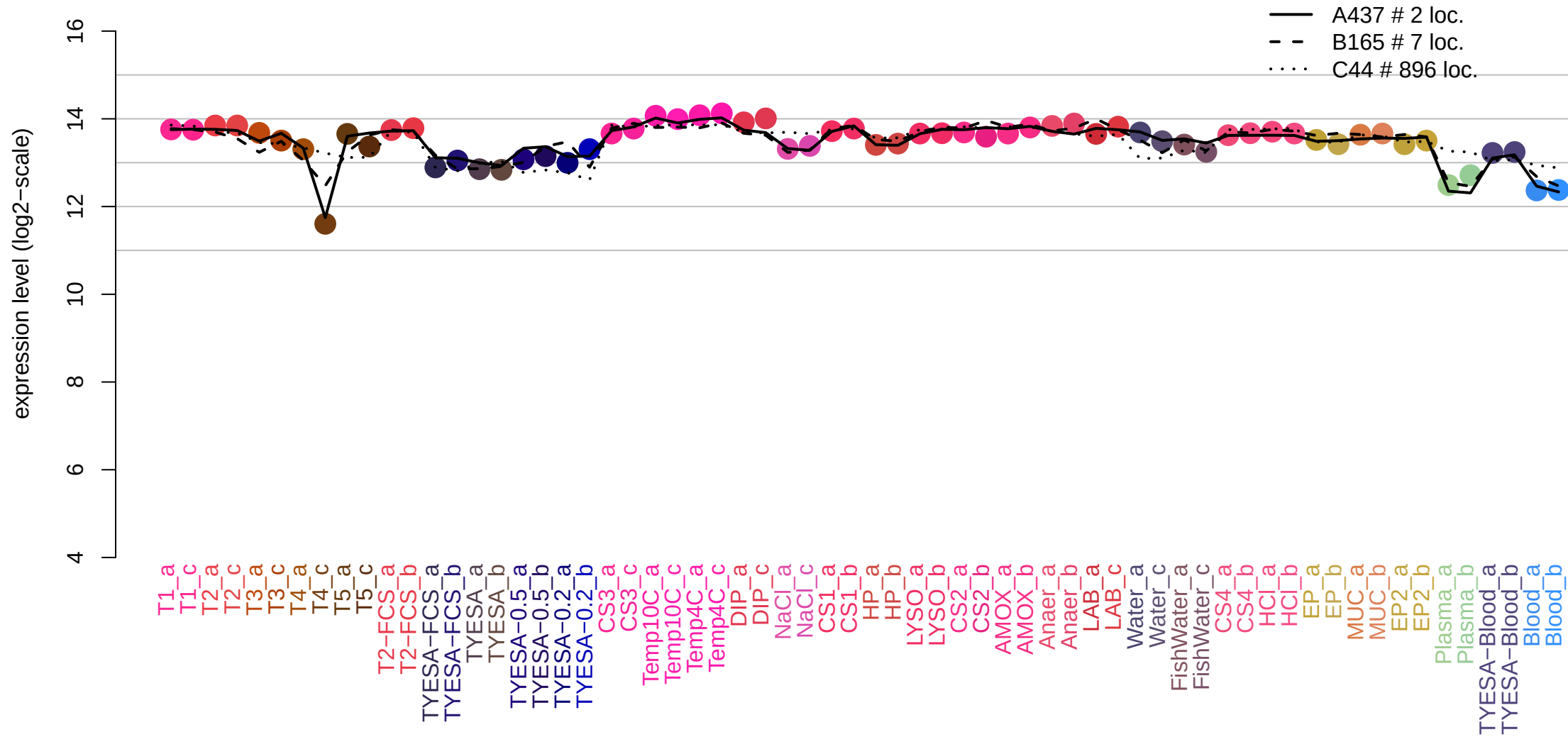
THC0290_1292 sucD (1491100,1491972,-1)
