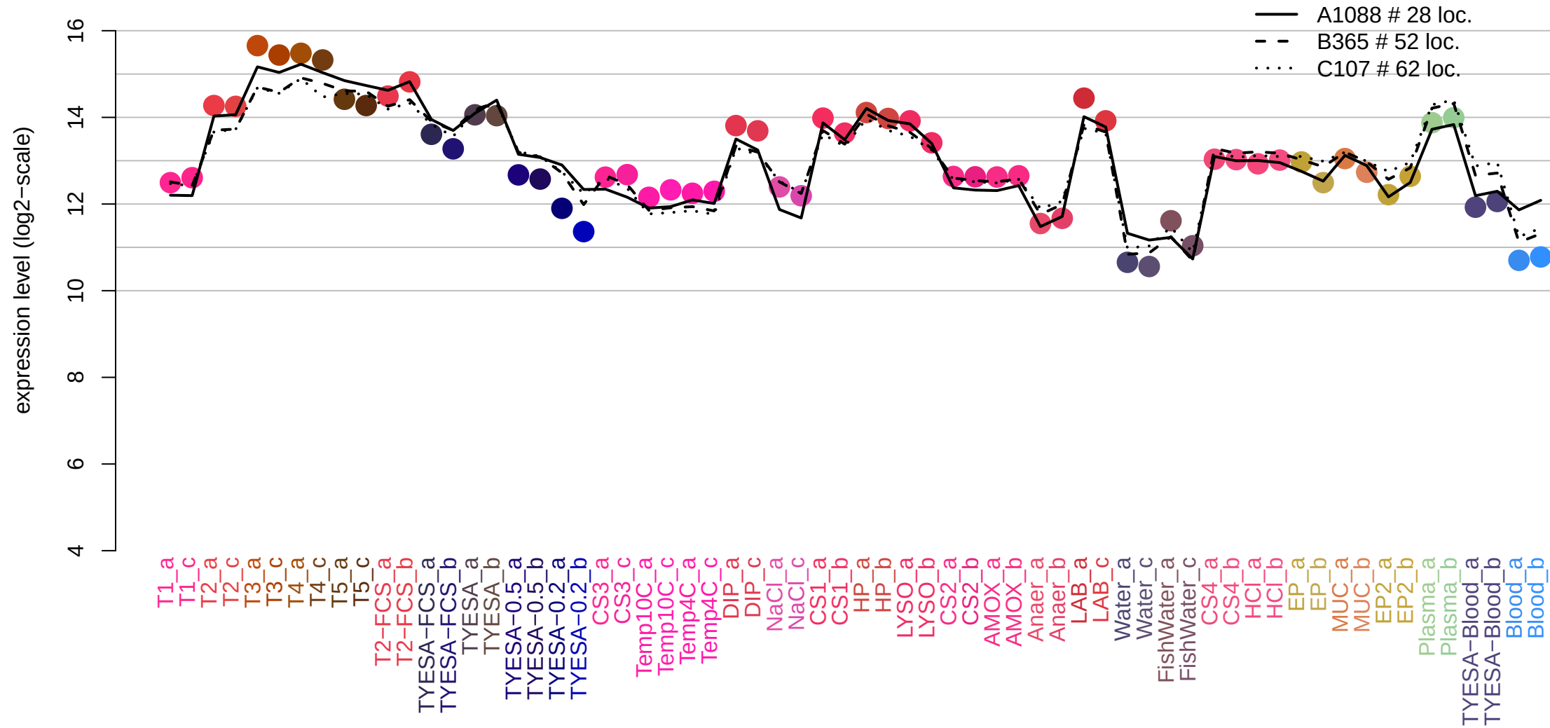
THC0290_1806 irpA (2090250,2091365,1)
