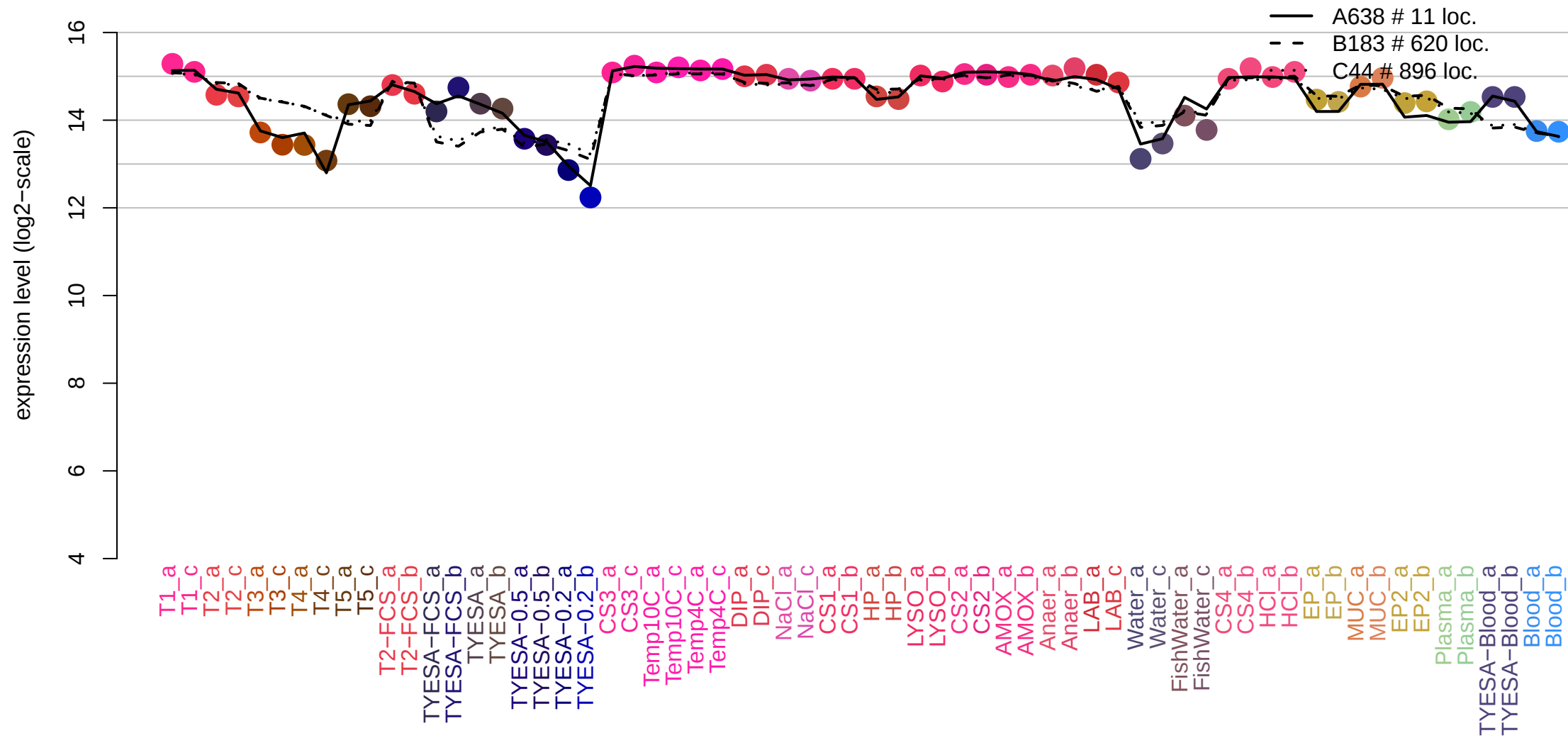
THC0290_1939 rplJ (2264685,2265185,-1)
