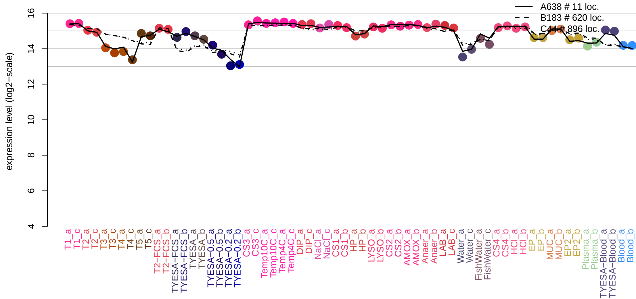
THC0290_1940 rplA (2265191,2265880,-1)
