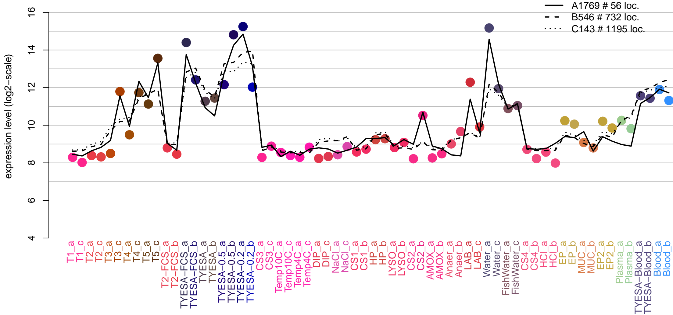
THC0290_miscRNA_0046 (1959533,1959661,1)
