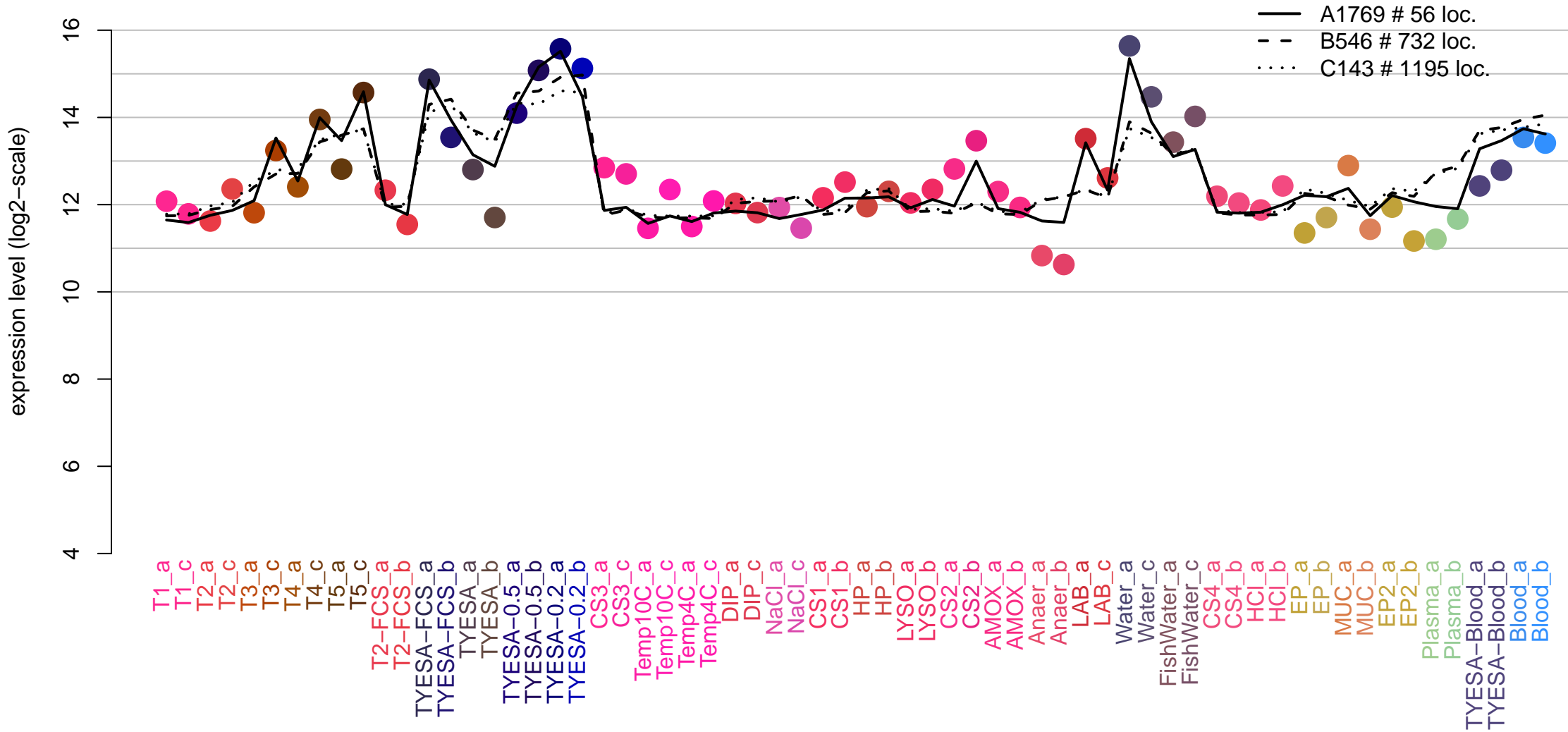
THC0290_tRNA_0026 (1681166,1681243,-1)
