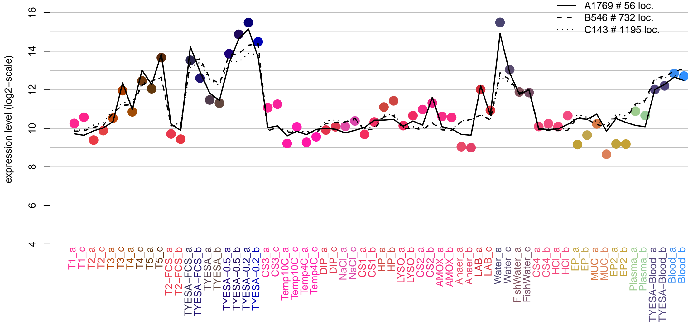
THC0290_tRNA_0034 (2003436,2003507,-1)
