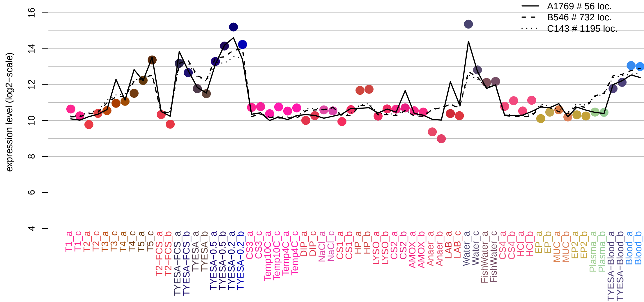
THC0290_tRNA_0041 (2267163,2267236,-1)
